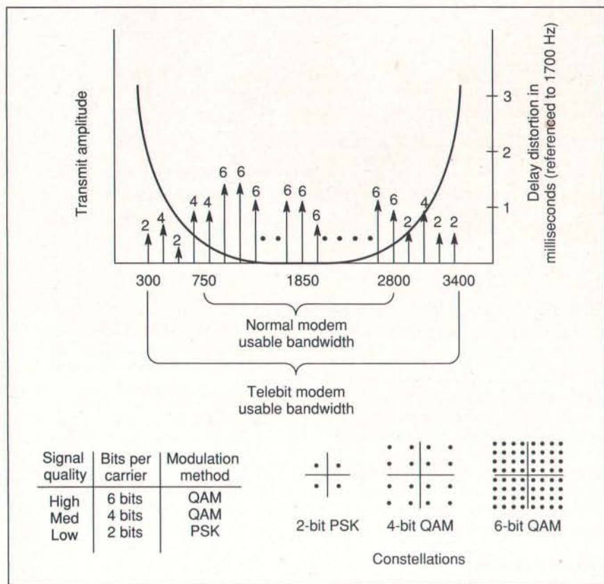
Figure 4: Telebit's Dynamically Adaptive Multicarrier Quadrature Amplitude Modulation encoding scheme. The Telebit Trailblazer modems use many small channels, modulated at low speeds, to make the best use of a phone line's available bandwidth. The signal quality of each 7.8-Hz channel determines what modulation scheme, if any, is used for that channel.
